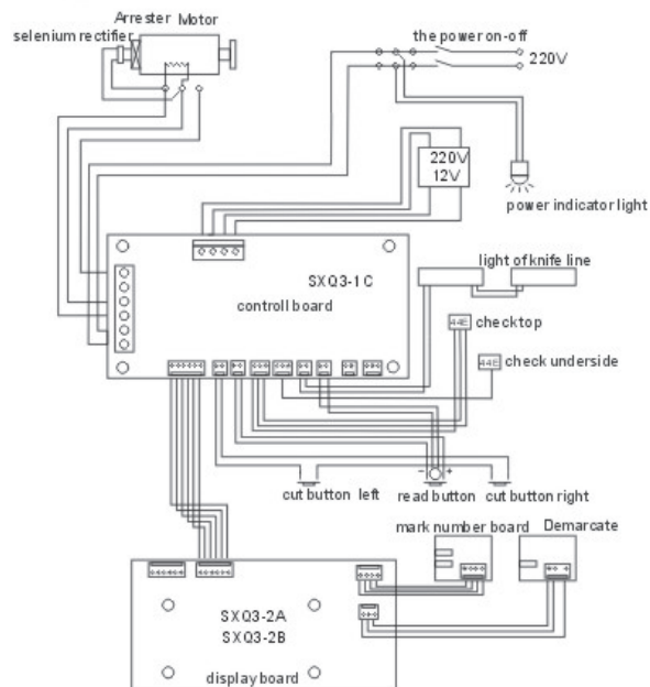
650 Digital cutting machine circuit line chart
